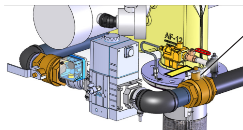
Gas Valve (shown in ON position)
