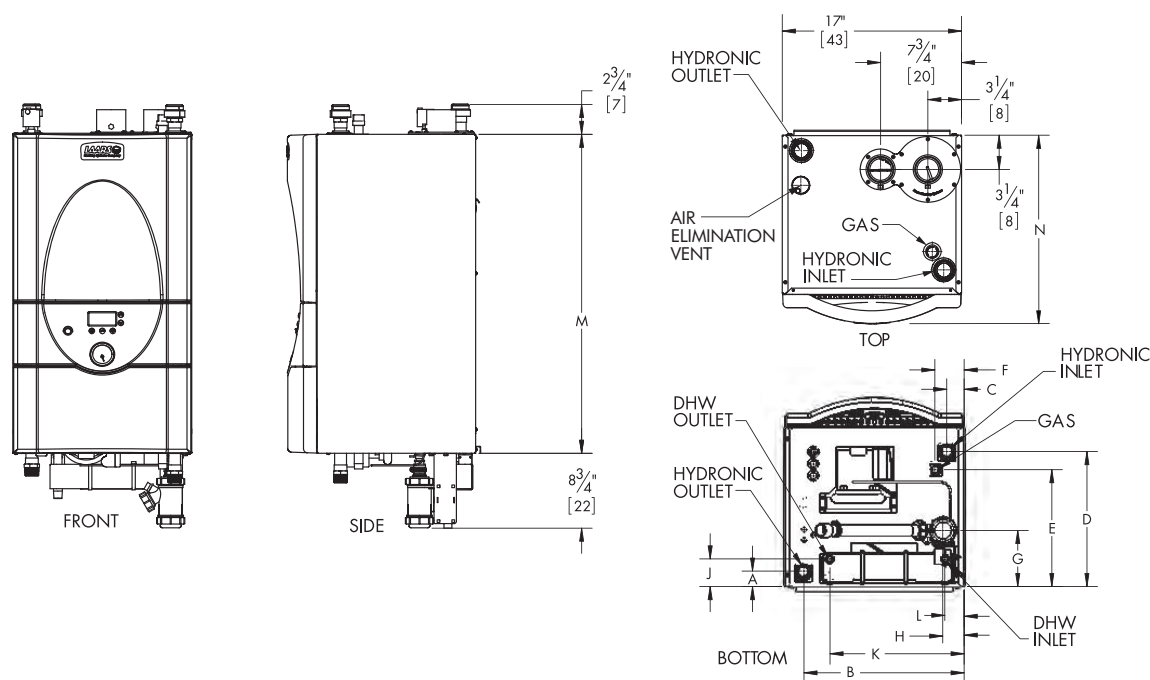
MASCOT LX Dimensions
