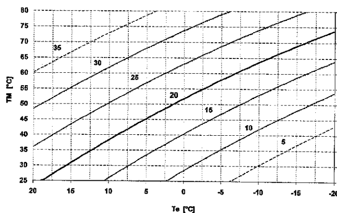
Graph 2 (Slope scale range for "kt" curve) Graphique 2
