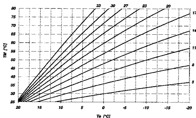
Graph 1 (Available "kt" curves) Graphique 1
