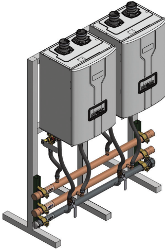
2-Unit Side-by-Side
