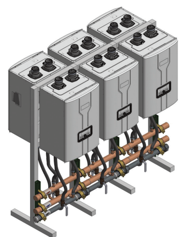
6-Unit Back-to-Back
