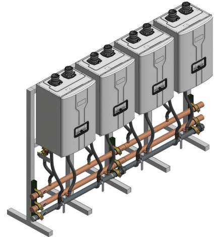
4-Unit Side-by-Side
