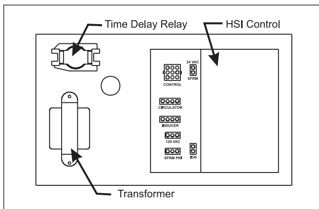
Figure 19. Control box.
