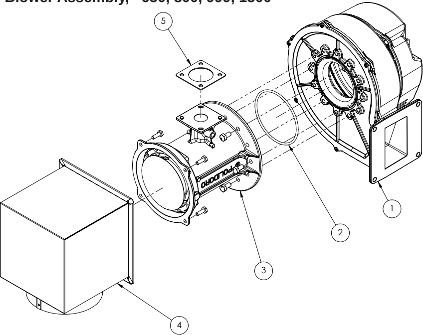
Blower Assembly, 650, 800, 999, 1500
