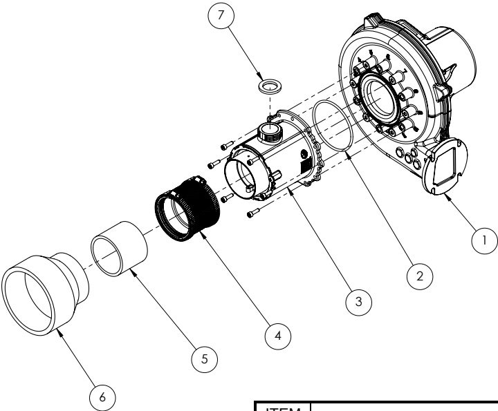
Blower Assembly, 399 & 500
