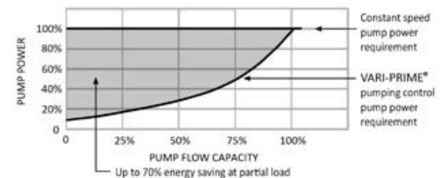
Typical Pump Power Savings via Vari-Prime
