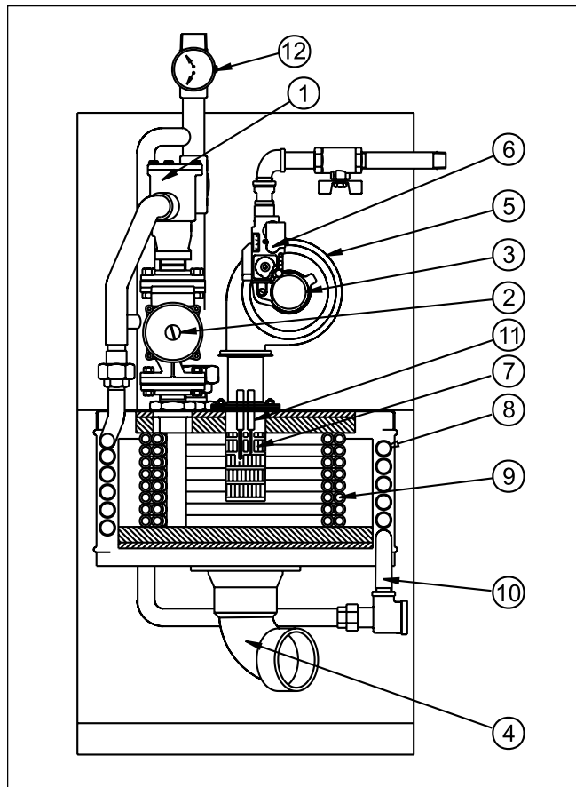
Figure 21. Parts Identification.
