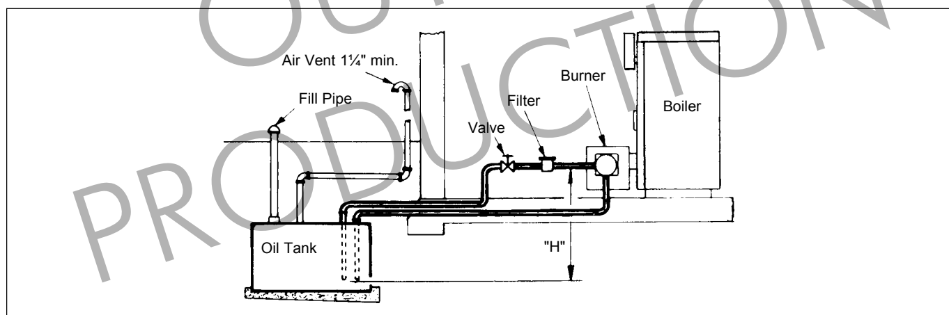
Figure 6. Two-Pipe System.
