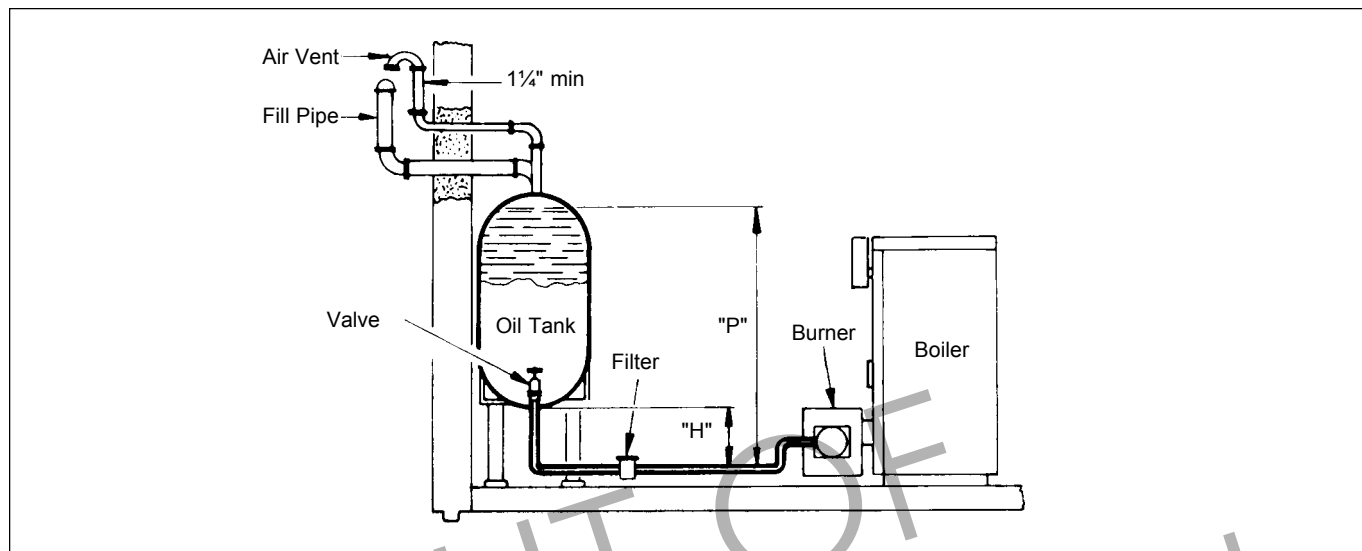
Figure 5. One-Pipe System.
