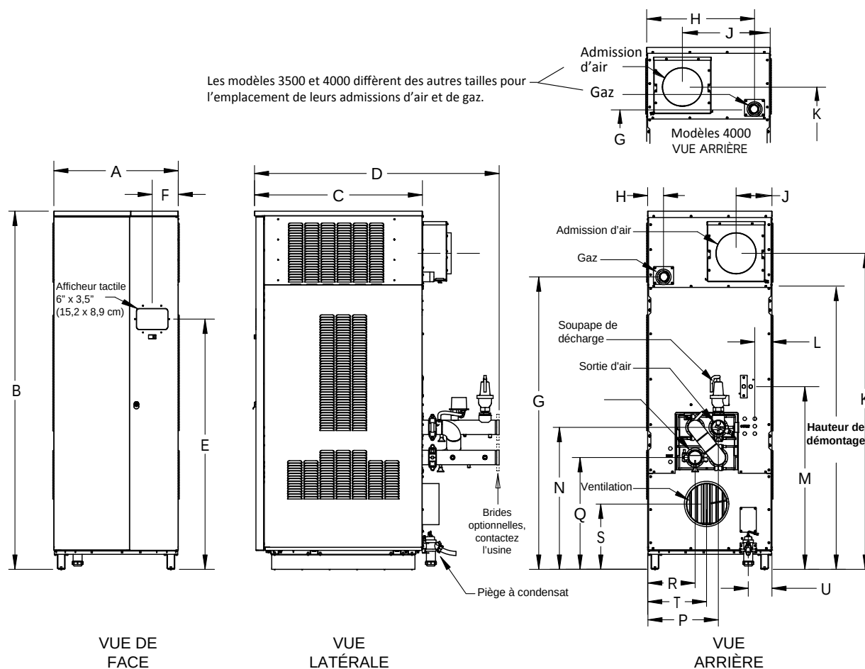
Figure 1. Dimensions
