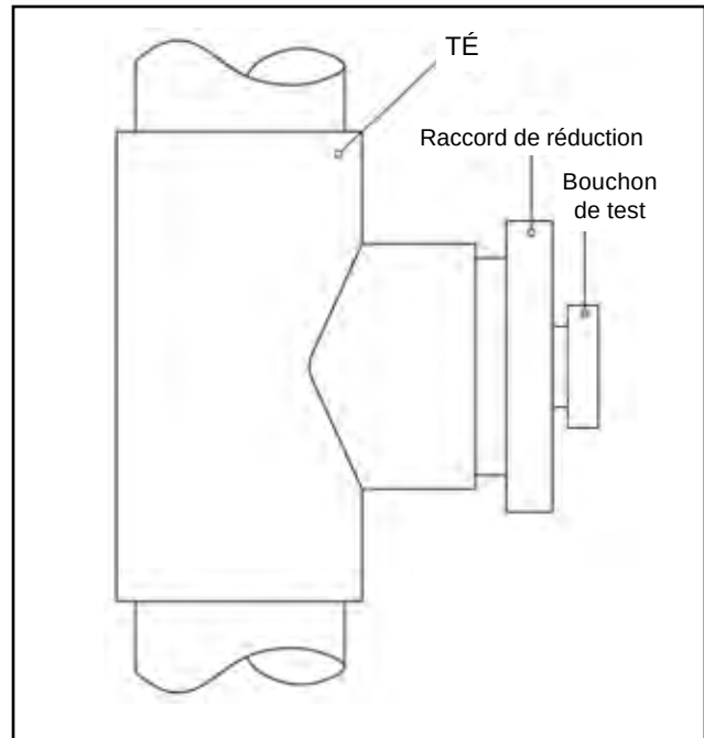
Figure 2. Point de test
