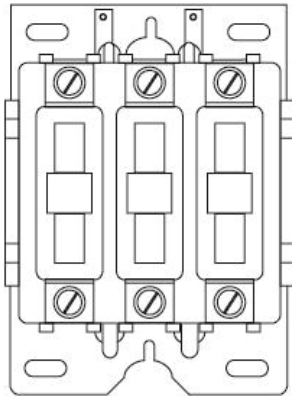
Fig. 7. Magnetic Contactor
